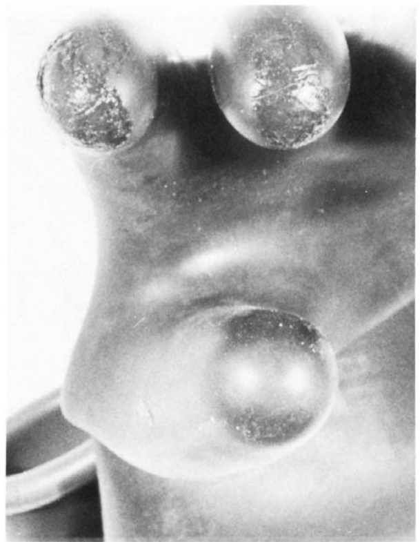
FIG. 12 Hard Spot
