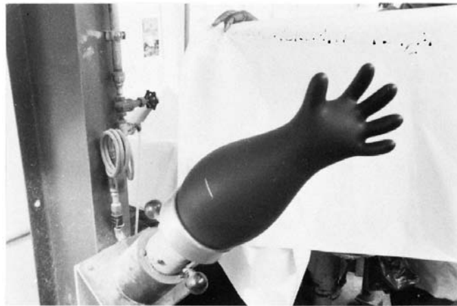
FIG. 37 Inflator (Glove Inflated to Maximum Allowable Degree)
