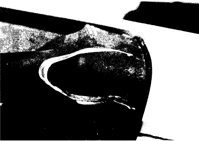
FIG. 19 Ozone Cracks
